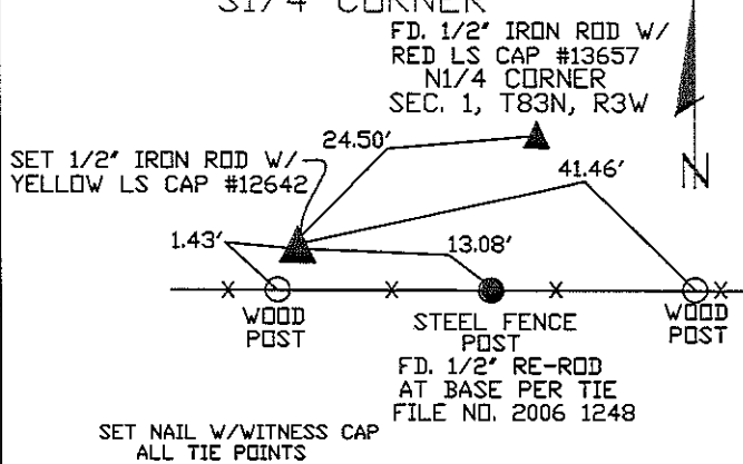
S1/4 CORNER
